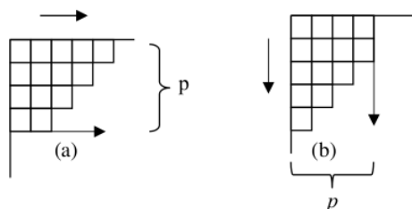
Figure 2. Young's table for p = 4 of paraboson (a) and parafermion (b).
