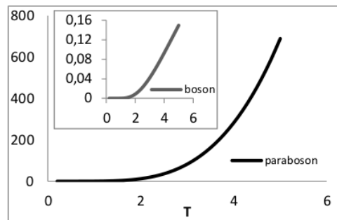
Figure 6. The average number of particles, N(T) , for paraboson system. Inset: the same quantity for boson.
