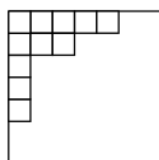
Figure 1. Young's table for \lambda = (5,3,1,1,1) .
